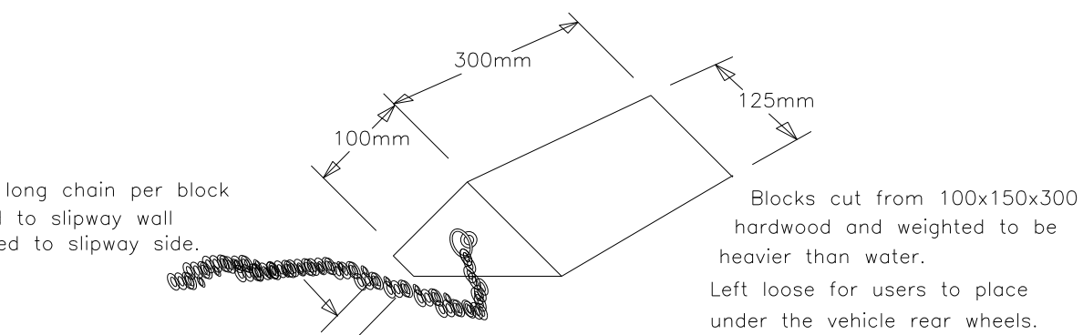
Detail of Chocks (2No required)
